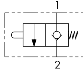
Hydraulic circuit
